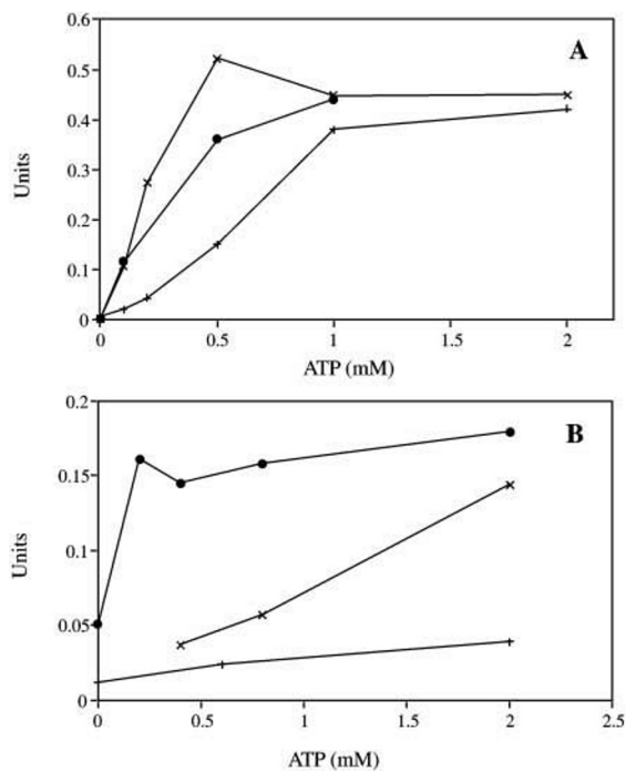
FIG. 7. Stimulation of CTP and GTP reduction by ATP. A, NrdD (3.6 μg) and NrdG (3.0 μg) were incubated under standard conditions for CTP reduction at increasing concentrations of ATP (+) or increasing concentrations of ATP + 0.1 mM dATP (●) or increasing concentrations of ATP + 0.1 mM dGTP (×). B, NrdD (3.6 μg) and NrdG (3 μg) were incubated under standard conditions for GTP reduction except for the effector. +, increasing concentrations of ATP alone; ×, increasing concentrations of ATP with 0.5 mM dTTP; ●, increasing concentrations of ATP with 0.5 mM dTTP + 0.2 mM dATP.
