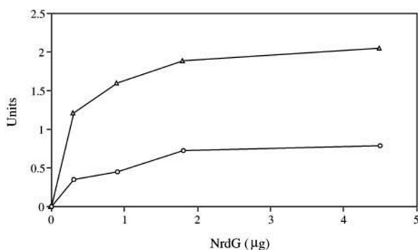
FIG. 6. Dependence of dCTP formation on the concentrations of NrdD and NrdG. Increasing amounts of reconstituted NrdG were incubated in the presence of 4 (○) or 8 (△) μg of NrdD under standard conditions, and the amount of dCTP formed was determined.
