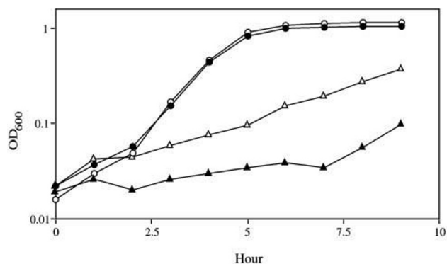
FIG. 1. Strict anaerobic growth of L. lactis requires the presence of active nrdD and nrdG . L. lactis subsp. cremonis MG1363, wild type, \circ , microaerobic growth; \bullet , strict anaerobic growth. L. lactis nrdD - : \Delta , microaerophilic growth; \blacktriangle , strict anaerobic growth. Growth was measured in M17 with 0.5% glucose.
