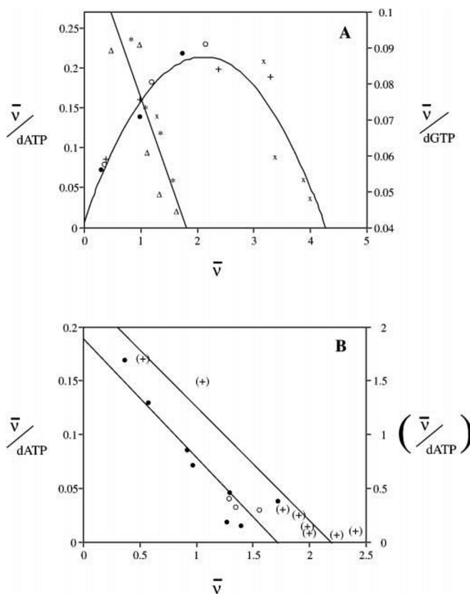
FIG. 8. A, binding of dATP and dGTP to NrdD (Scatchard plots). dATP binding (●, ○, +, ×) was measured (32) in separate experiments with four different preparations of NrdD. \bar{\nu} is molecules of nucleotide bound per NrdD dimer. dGTP binding (△, *) was measured with two of the four NrdD preparations. B, dATP binding in the presence of 1 mM dGTP (+) or 2 mM ATP (●, ○). Note the differences in scales on the two ordinates ( left = ATP, right = dGTP).
